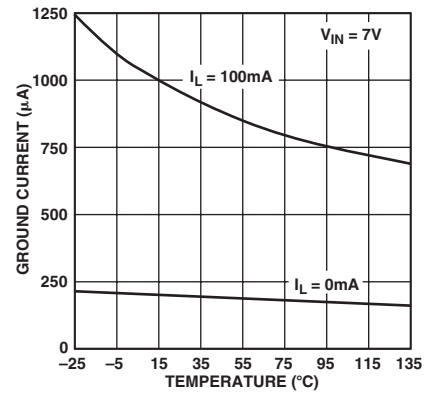
TPC 6. Quiescent Current vs. Temperature
