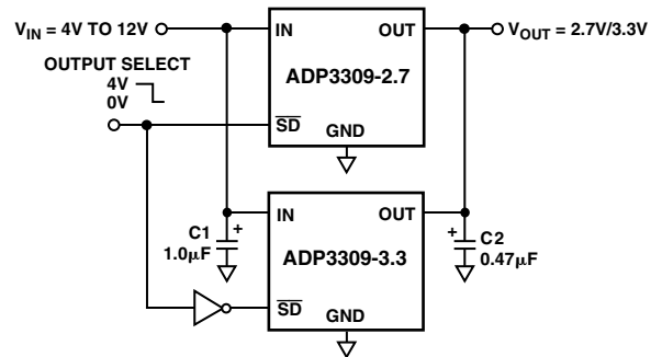
Figure 3. Crossover Switch
